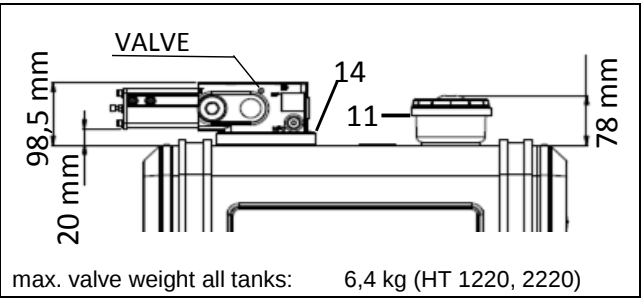
Valve mounted on tank
