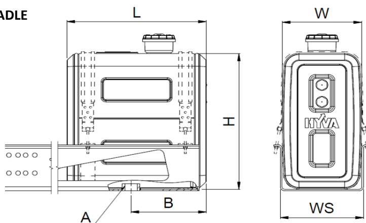
TANK + SUPPORT ON CRADLE
