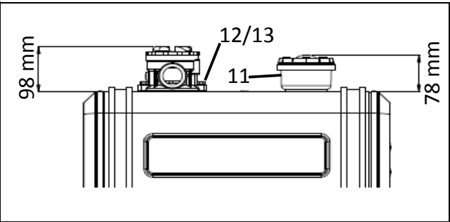
Chassis or cylinder (SAE) mounted valve
